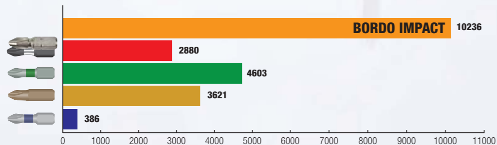
PH2 x 50MM CYCLES BEFORE FAILURE average impact 10.3 Nm at 100% loading
