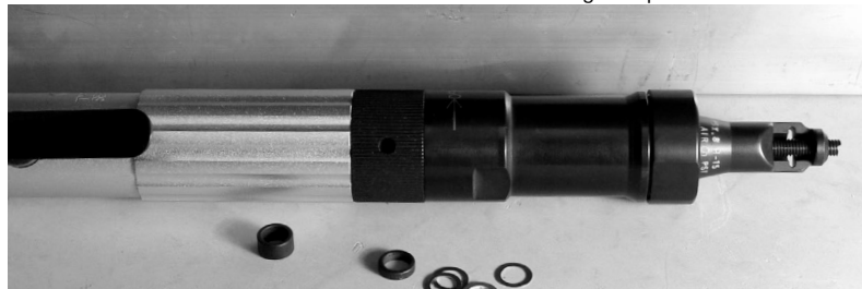
Front end assembly with longest spacer to suit 1.0D insert and shim washer.
